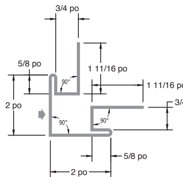
304 Outside Corner
