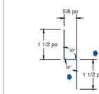
Z-58 Couvre-joint de support
